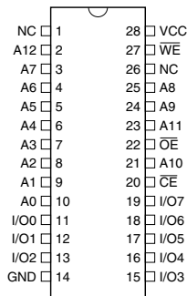
PDIP, SOIC Top View
